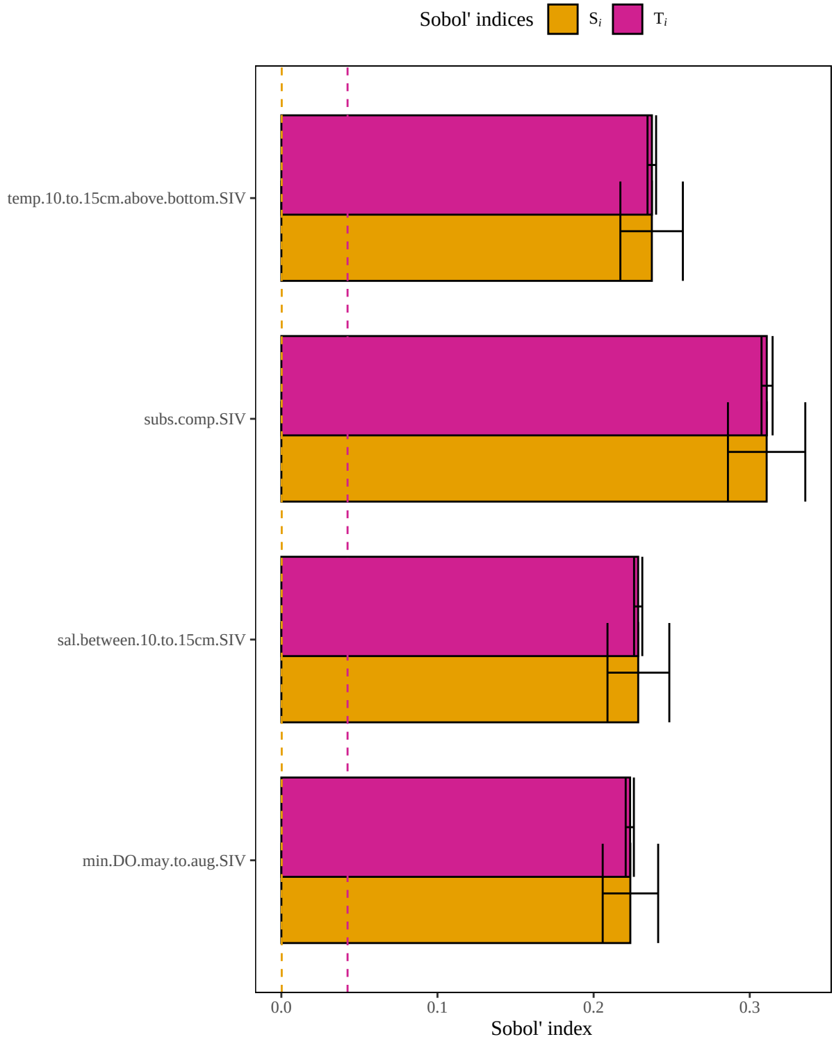
Figure 4. Results of a sensitivity analysis for the flounderSouthern model based on an arithmetic mean structure. Dashed lines represent baseline numerical approximation error for S_i and T_i ( i.e. , dummy variables).
